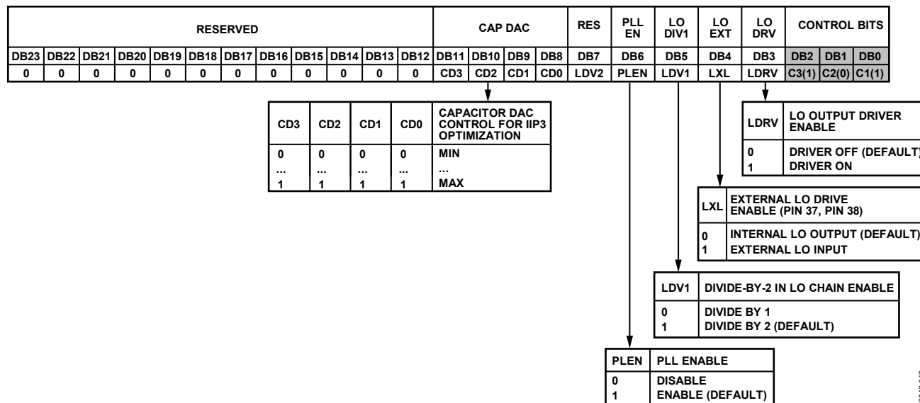
Figure 43. Register 5—PLL Enable and LO Path Control Register Map
