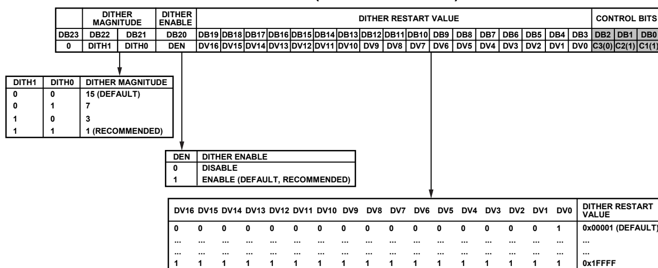
Figure 41. Register 3—Σ-Δ Modulator Dither Control Register Map
