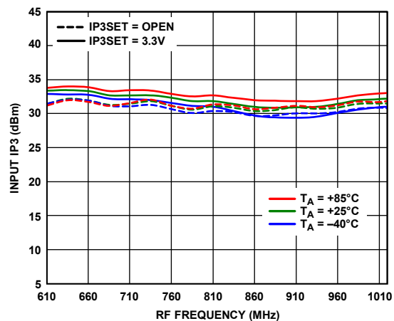
Figure 7. Input IP3 vs. RF Frequency
