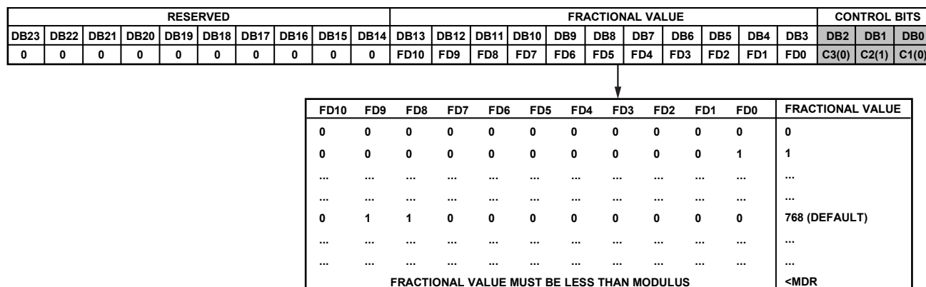
Figure 40. Register 2—Fractional Divide Control Register Map
